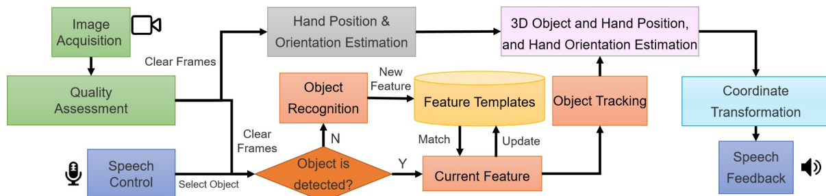
Fig. 6. System workflow.
