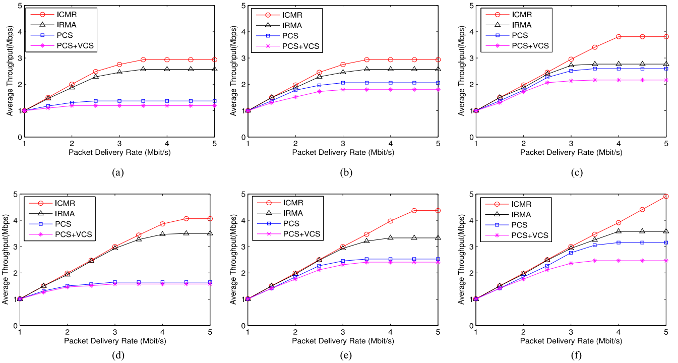
Fig. 14. Average throughput in terms of packet delivery rate in the random topology, under three transmission rates and two packet lengths. (a) l_p = 500 bytes, d = 100 m. (b) l_p = 500 bytes, d = 200 m. (c) l_p = 500 bytes, d = 400 m. (d) l_p = 2000 bytes, d = 100 m. (e) l_p = 2000 bytes, d = 200 m. (f) l_p = 2000 bytes, d = 400 m.
